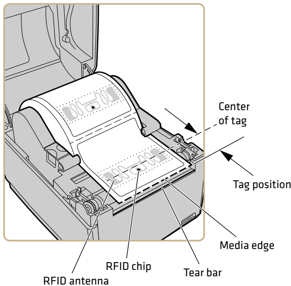
RFID Tag Position
